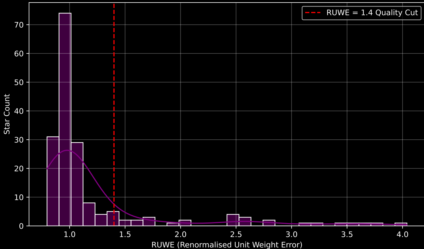
GAPOGEE DR17 Field [109+68_MGA] RUWE Distribution (n= 177)
