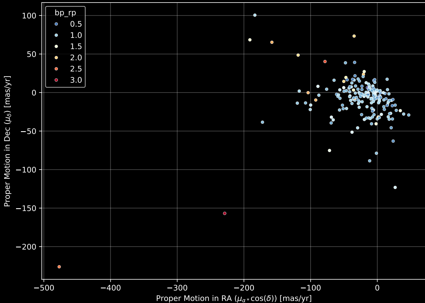
APOGEE DR17 Field: [109+68_MGA] Proper Motion Diagram (n= 190)
