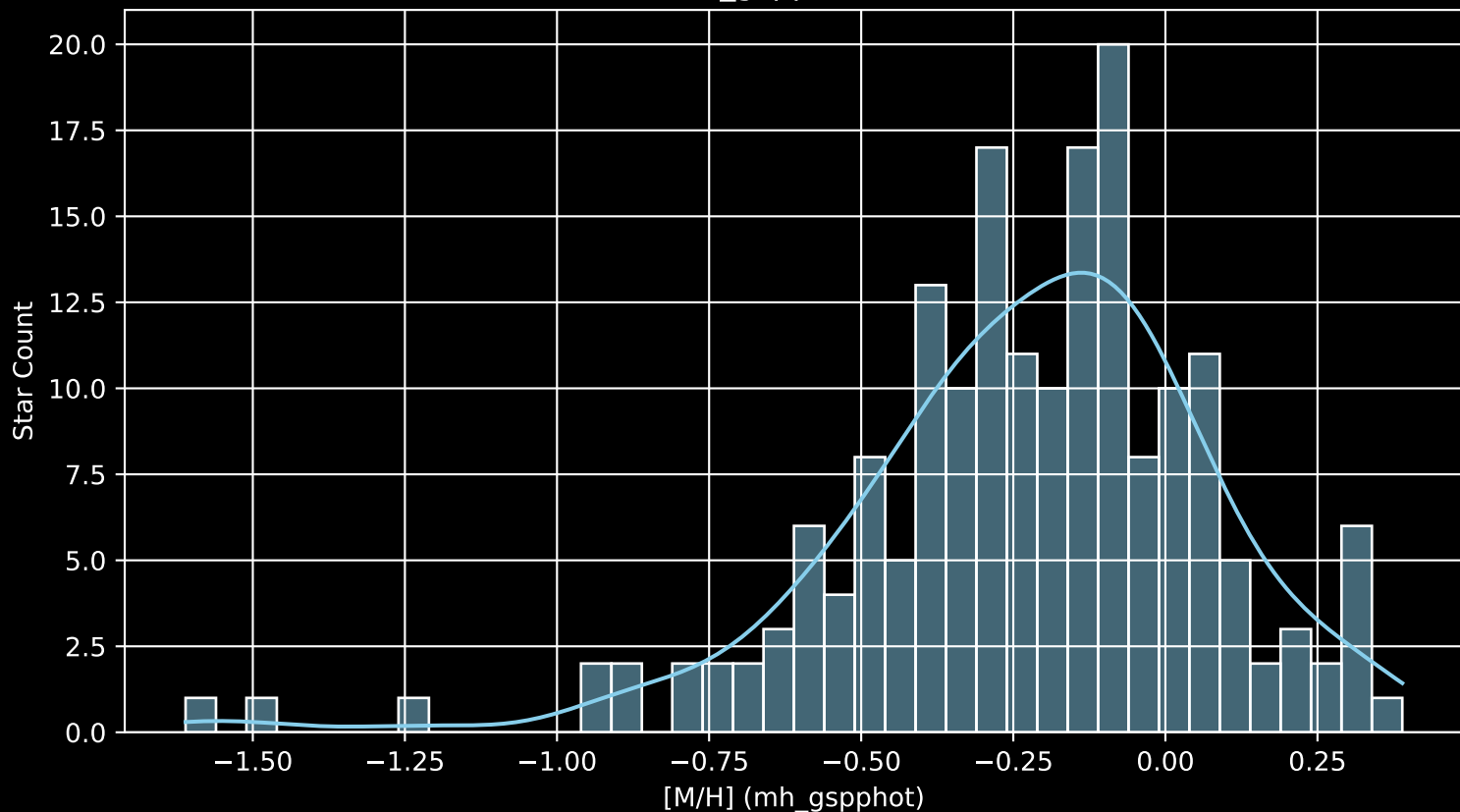
APOGEE DR17 Field: [109+68_MGA [M/H] (mh_gspphot) (n= 185)
