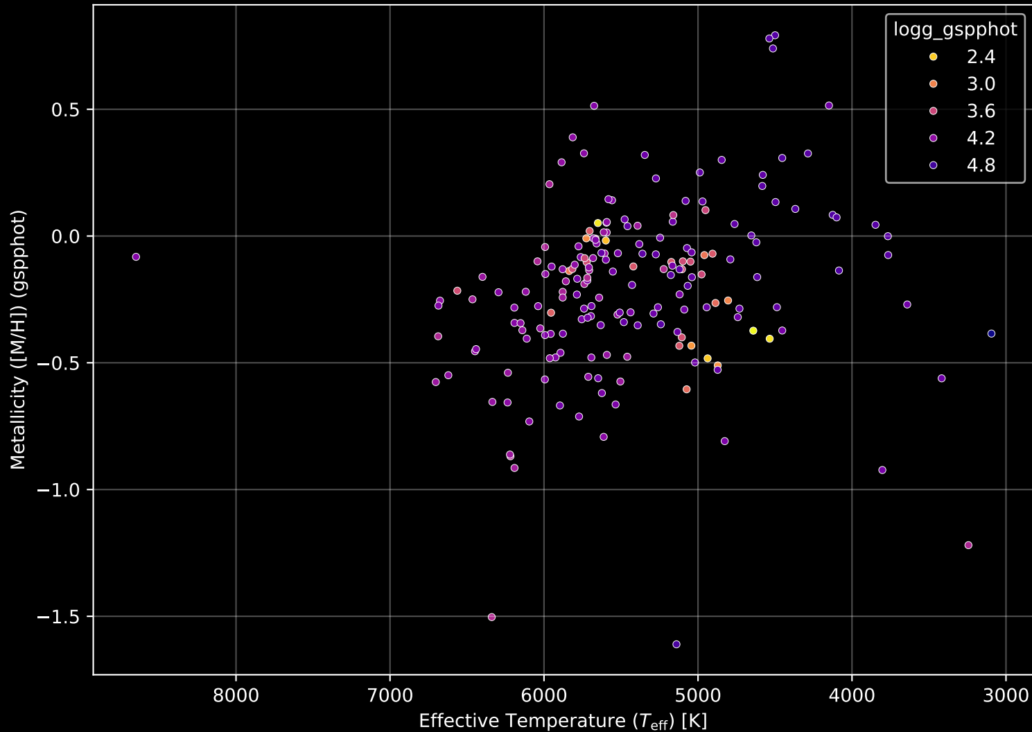
APOGEE DR17 Field: [109+68_MGA] Stellar Population Parameters (n= 190)
