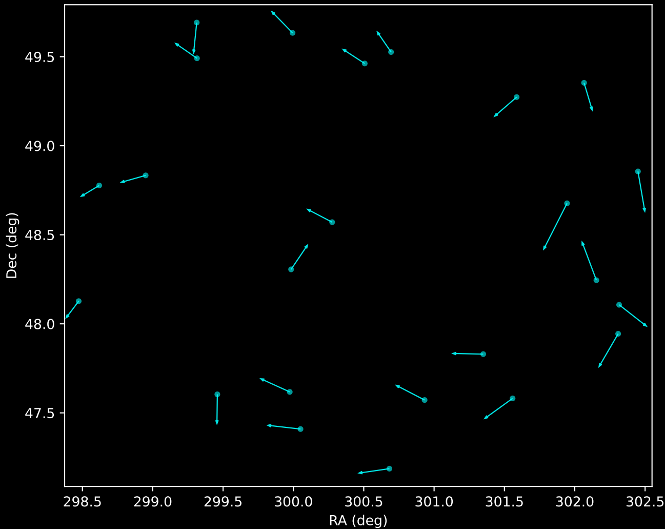
APOGEE DR17 Noise Stream Proper Motion Vectors (n=24)
