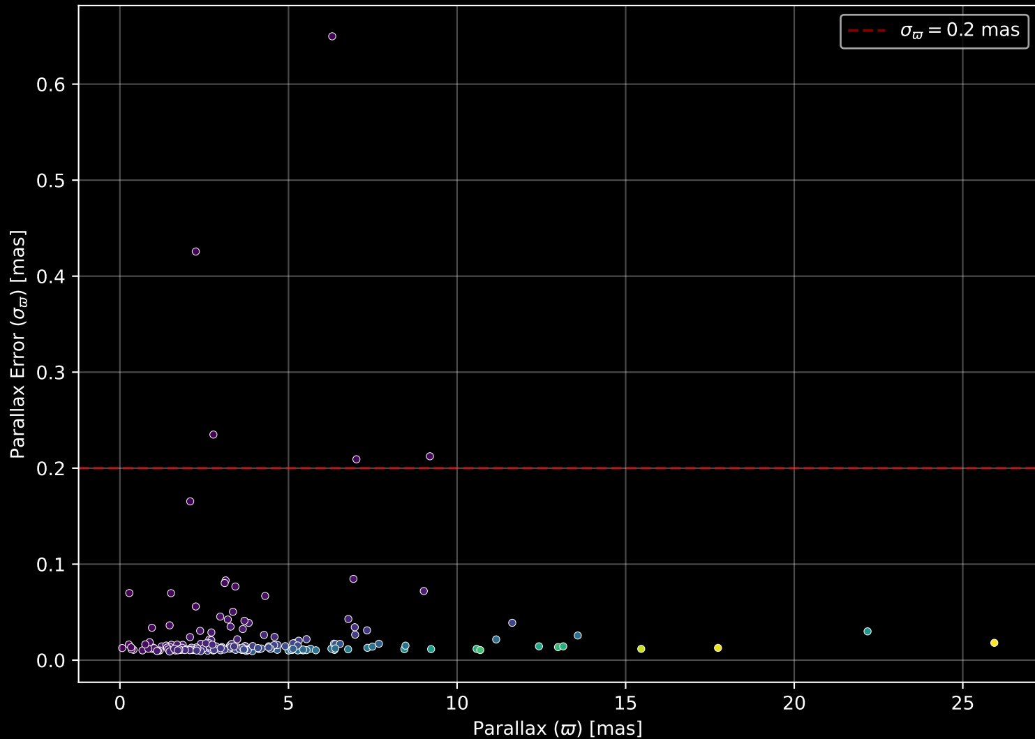
APOGEE DR17 Field: [109+68_MGA] Parallax Quality (n= 190)
