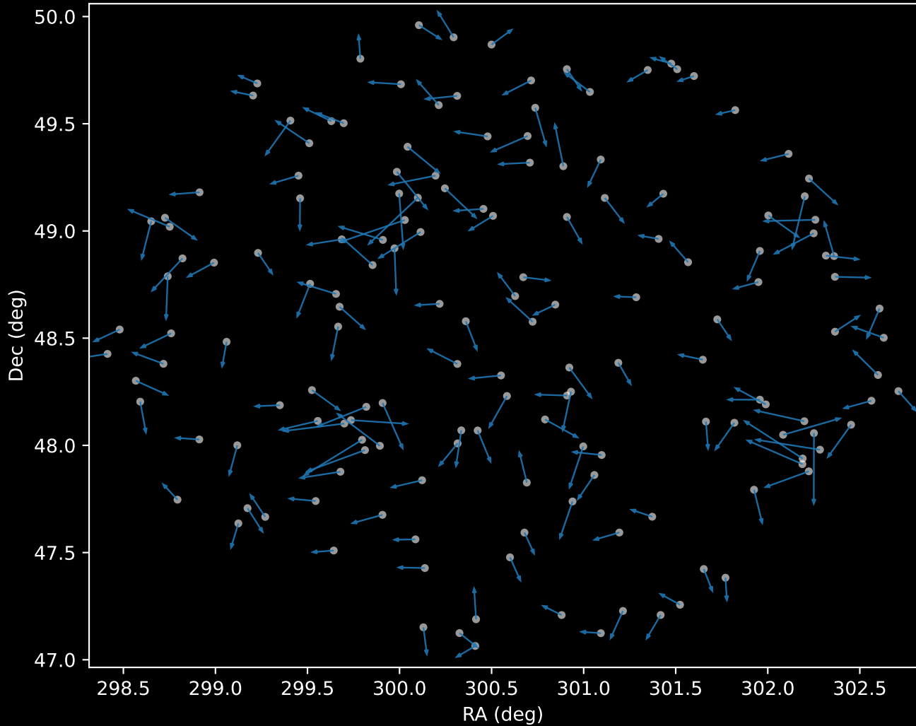
APOGEE DR17 Cluster 0 Proper Motion Vectors (n=160)
