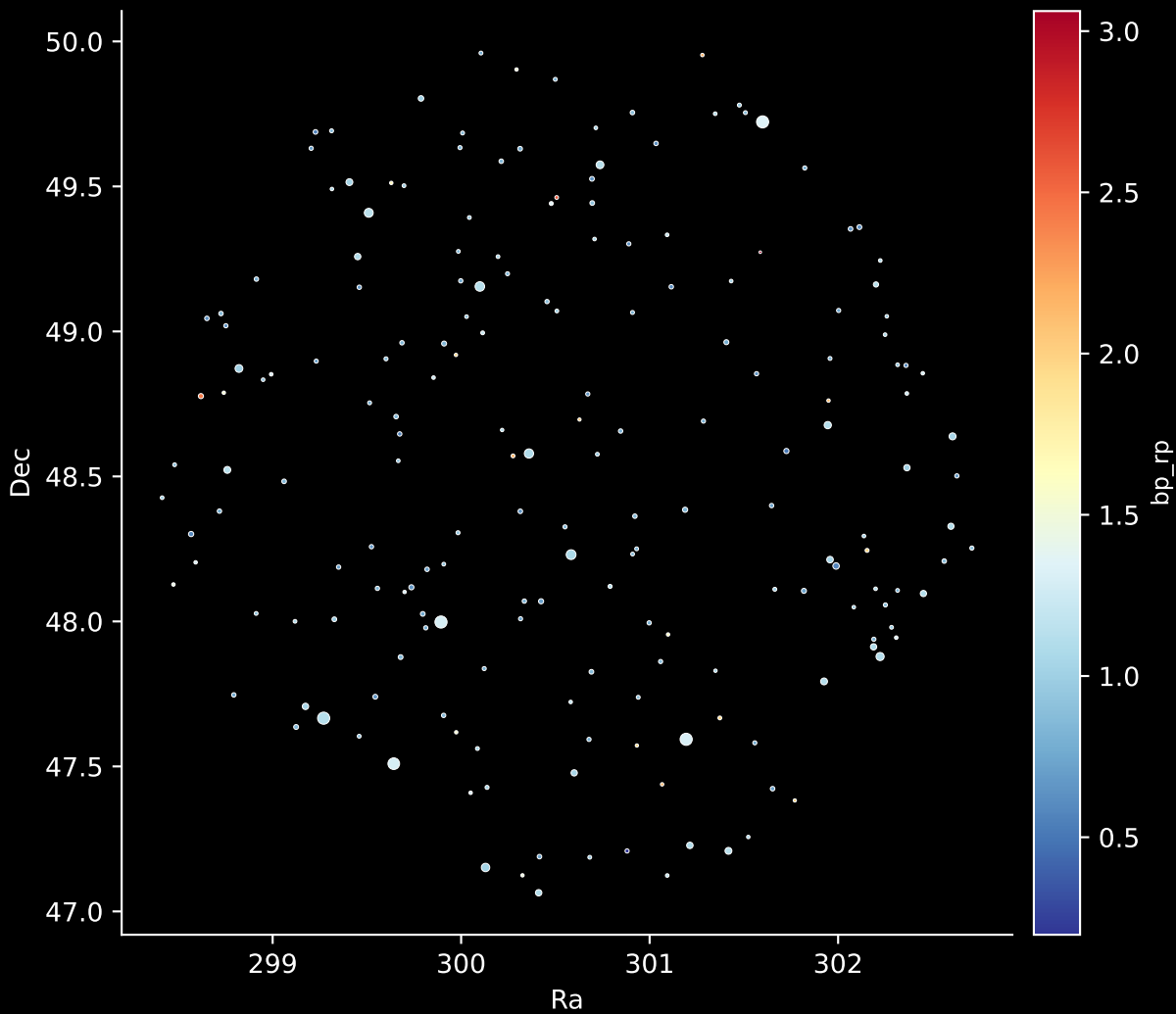
APOGEE DR17 Field: [109+68_MGA] Stars: 190
