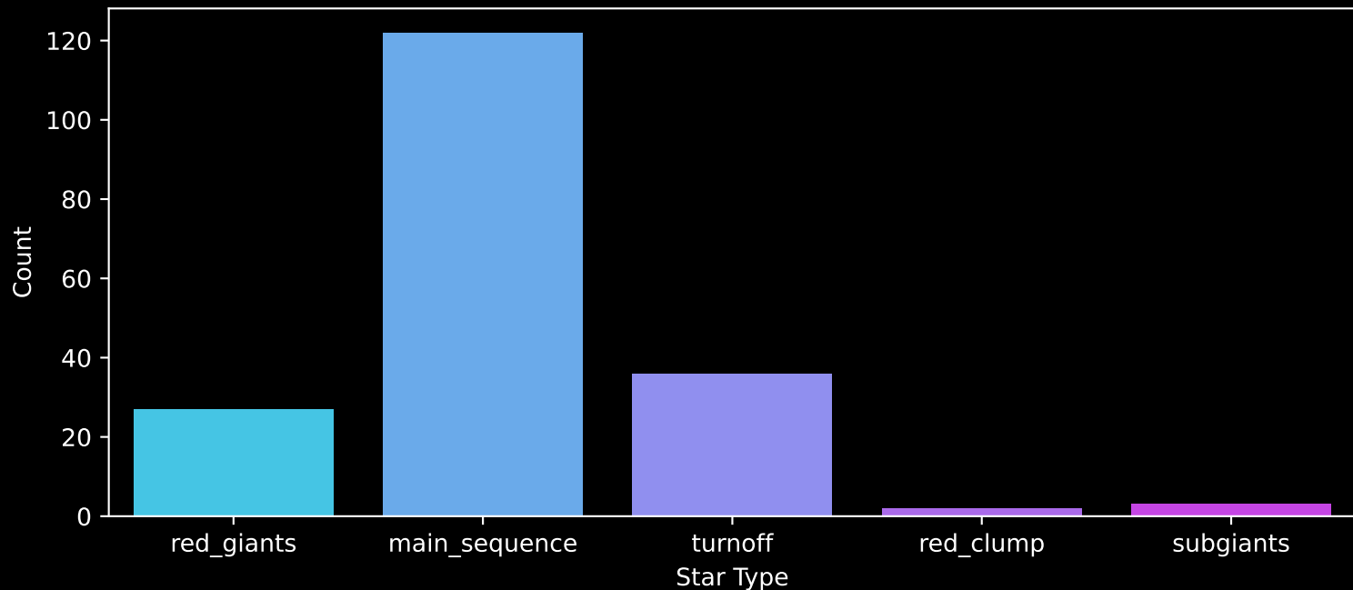
APOGEE DR17 Field: [109+68_MGA] Count plot of Star Type
